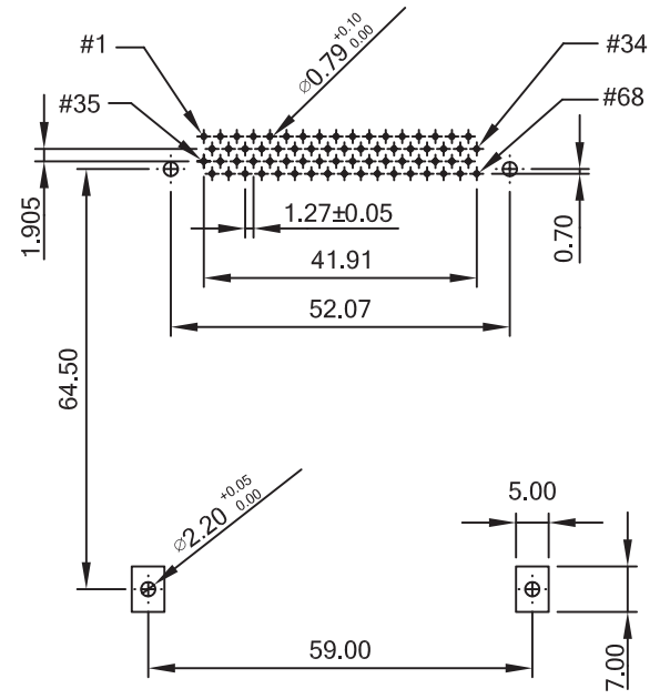
PCB LAYOUT: COMPONENT SIDE PCB THICKNESS: 1.60±0.00
