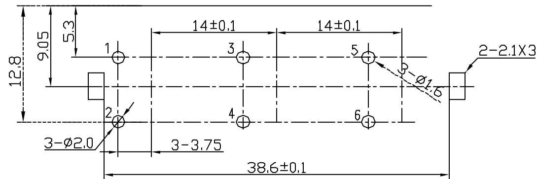
Dimensions of PC board hole(Commend) Bottom View
