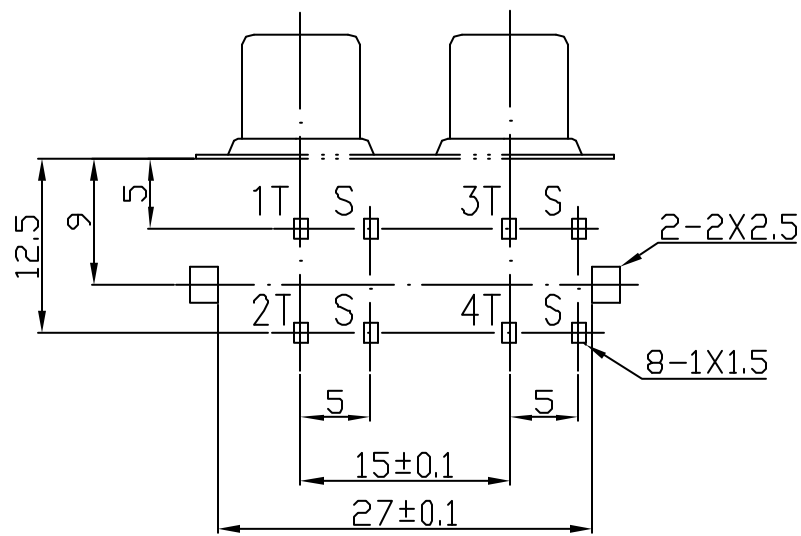
Dimensions of PC board holes(Commend) Bottom View
